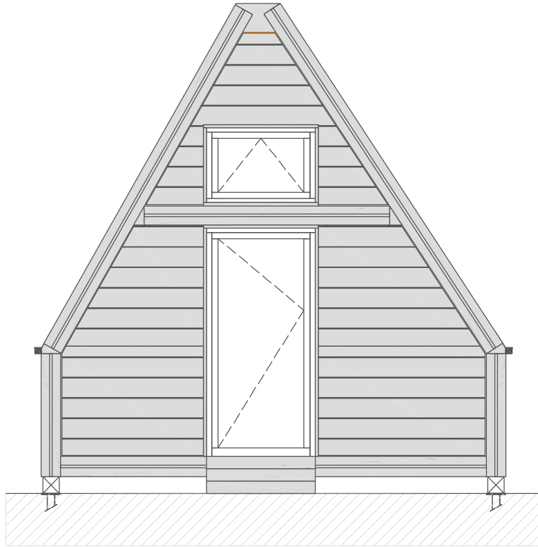
FRONT FACADE architectural drawing
