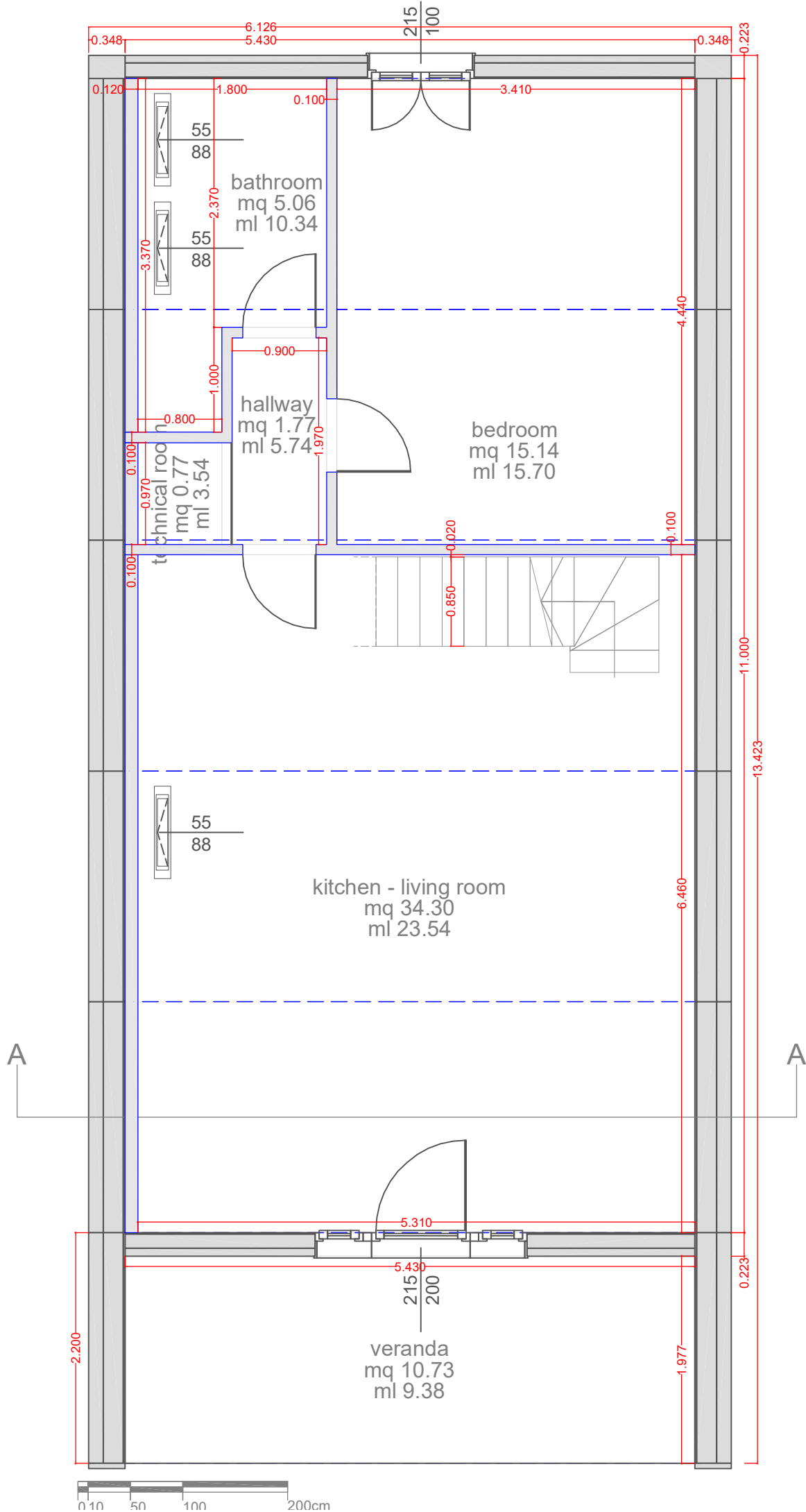
GROUND FLOOR architectural drawing
